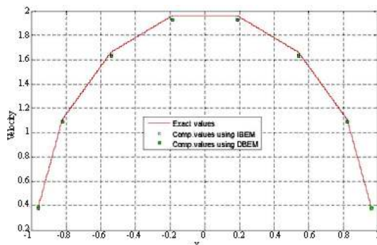
Graph 2: Comparison of computed and analytical velocity distributions over the boundary of a circular cylinder using 16 boundary elements with linear variation. The improvement gained by using 32 linear boundary elements can be seen from the following table.
