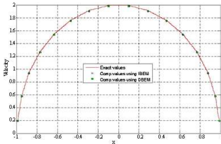
Graph 3: Comparison of computed and analytical velocity distributions over the boundary of a circular cylinder using 32 boundary elements with linear variation.
