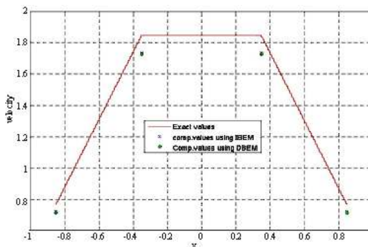
Graph 1: Comparison of computed and analytical velocity distributions over the boundary of a circular cylinder using 8 boundary elements with linear variation. The improvement gained by using 16 linear boundary elements can be seen from the following table.
