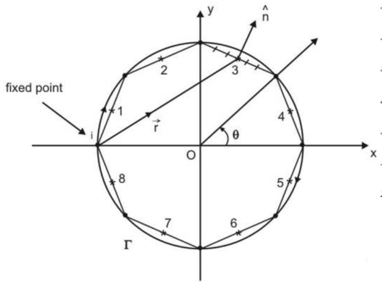
Fig. 2: shows the discretization of the circular cylinder of unit radius into 8 linear boundary elements.
