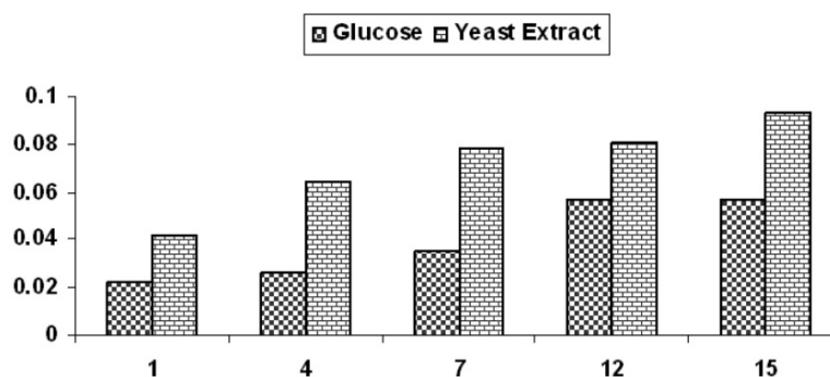
Fig. 4: Esterase activity (OD) in culture filtrate of B. thuringiensis (MOS-5) containing malathion and supplied with two different growth substrates.
