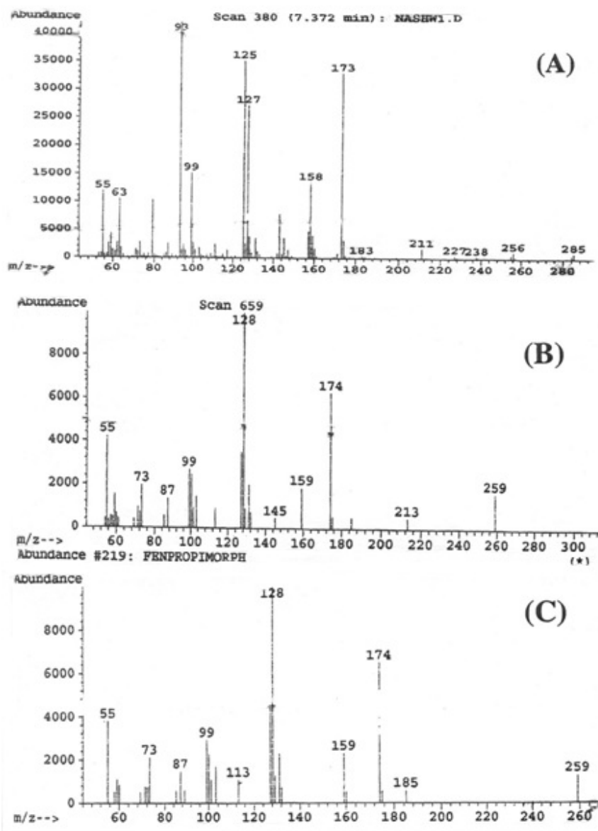
Fig. 3: (A) Mass spectrum chart of malathion, (B) Mass spectrum of malathion monoacid and (C) Mass spectrum of malathion diacid
