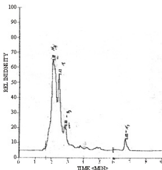
Fig. 2b: HPLC chart showing analysis of the metabolites extracted from MOS-5 liquid culture after 7 days incubation.
