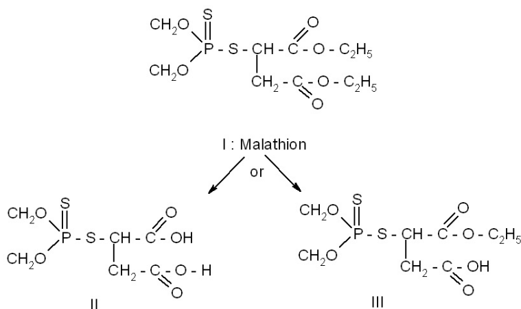
Fig. 5: The degradation products of malathion (I) into malathion di-acid (II) and malathion mono (III) acids.
