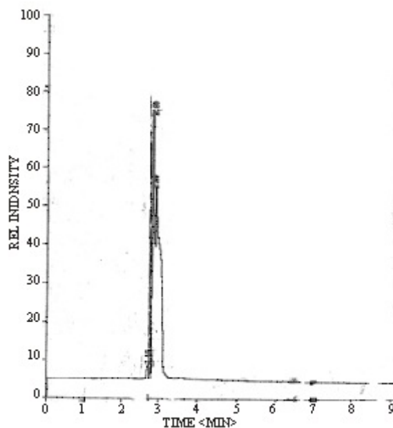
Fig. 2a: HPLC chart of Standard malathion
