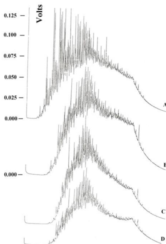
Fig 2: A : Gas Chromatograms showing the resolved PAHs at the beginning of the experiment (0-time). B : Gas Chromatograms showing patterns of the residual PAHs extracted from the rhizosphere of Triticum aestivum after 60 days. C : Gas Chromatograms showing patterns of the residual PAHs extracted from the rhizosphere of Zea mays after 60 days. D : Gas Chromatograms showing patterns of the residual PAHs extracted from the rhizosphere of Vicia faba after 60 days.
