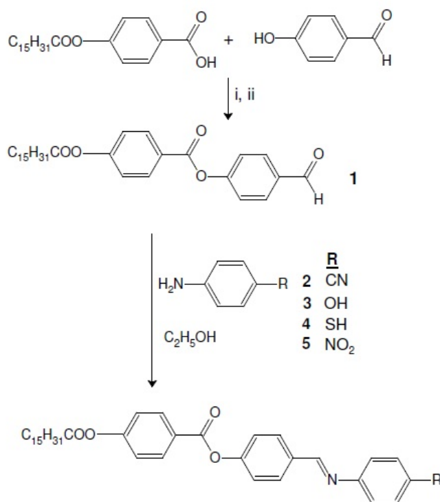
Scheme 1: Synthetic routes towards the formation of intermediates and target compounds 6-9 . Reagent and conditions: (i) \text{SOCl}_2 , reflux for 3 hours; (ii) anhydrous \text{CH}_2\text{Cl}_2 , DMF, (\text{C}_2\text{H}_5)_3\text{N} , \text{N}_2 atmosphere, reflux for 5 hours.
