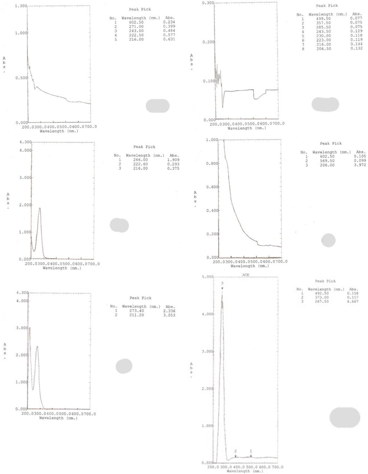
Fig. 3: The absorption rate of some photoprotectants to UV-light using Spectrophotometer at the wavelength range of 200-700nm. vii) Selenium, viii) Titanium dioxide, ix) Vitamin (A+E) mixture, x) Vitamin (A+C) mixture, xi) Vitamin (E+C) mixture, xii) Vitamin (A+E+C) mixture.
