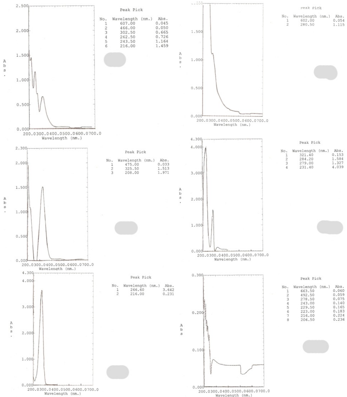
Fig. 2: The absorption rate of B. thuringiensis var. kurstaki (HD-73) and some photoprotectants to UV-light using Spectrophotometer at the wavelength range of 200-700nm.
