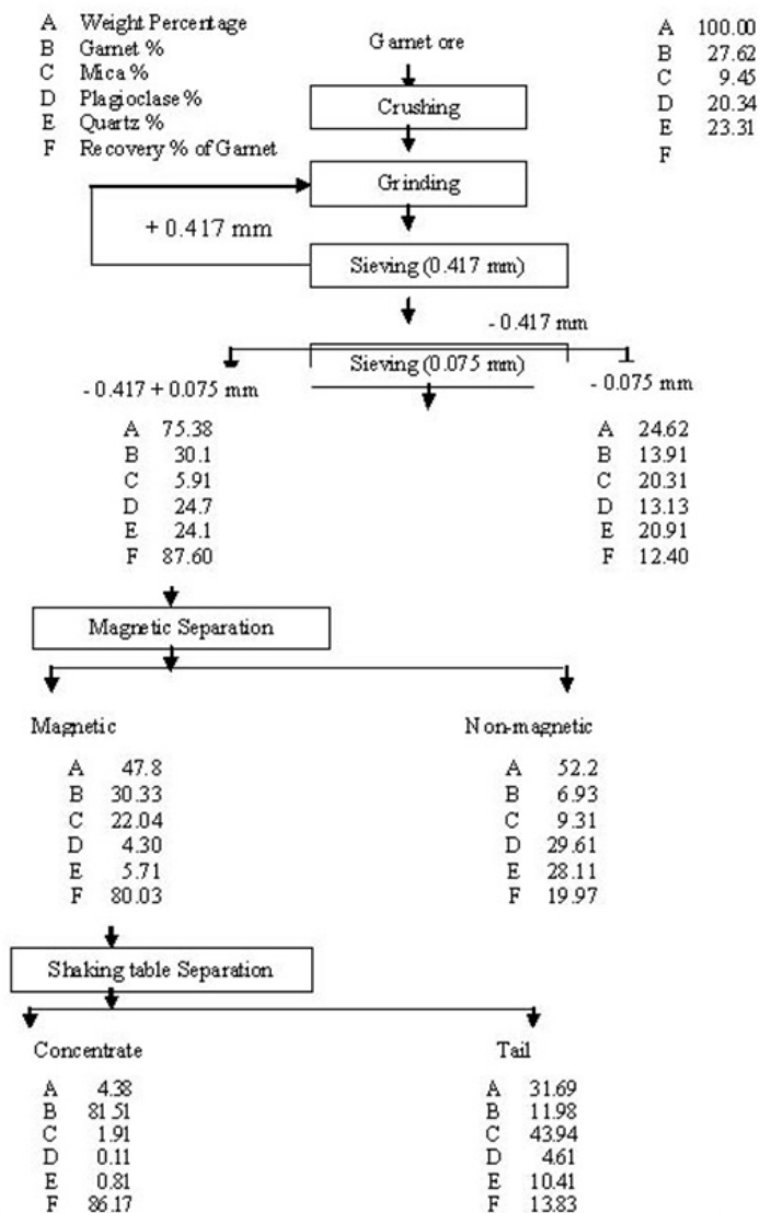
Fig. 9: Flowsheet of garnet ore material.
