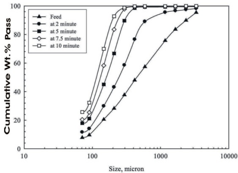
Fig. 6a: Effect of grinding time on garnet.
