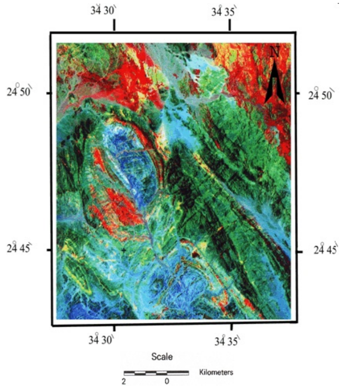
Fig. 1: Landsat TM ratio image (bands 5/7, 5/1, and band 4 in RGB) for the study area; illustrates the lithology as follows: ultramafics: (red), psammitic gneisses: (dark green), foliated metagabbros (light green) garnet-biotite schist: (purple) and granitic rocks: (bluish green).
