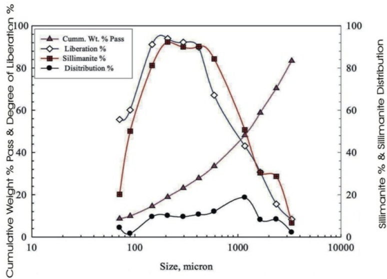
Fig. 3: Size analysis and liberation studies of sillimanite.
