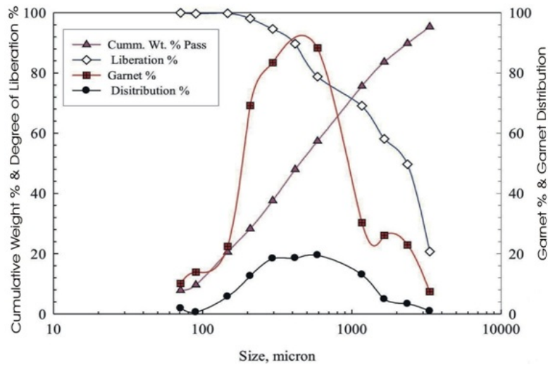
Fig. 4: Size analysis and liberation studies of garnet.
