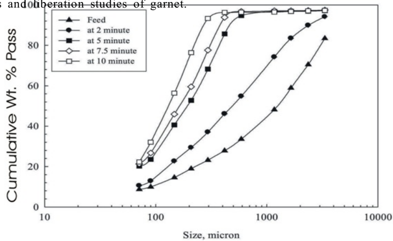
Fig. 4: Size analysis and liberation studies of garnet.
