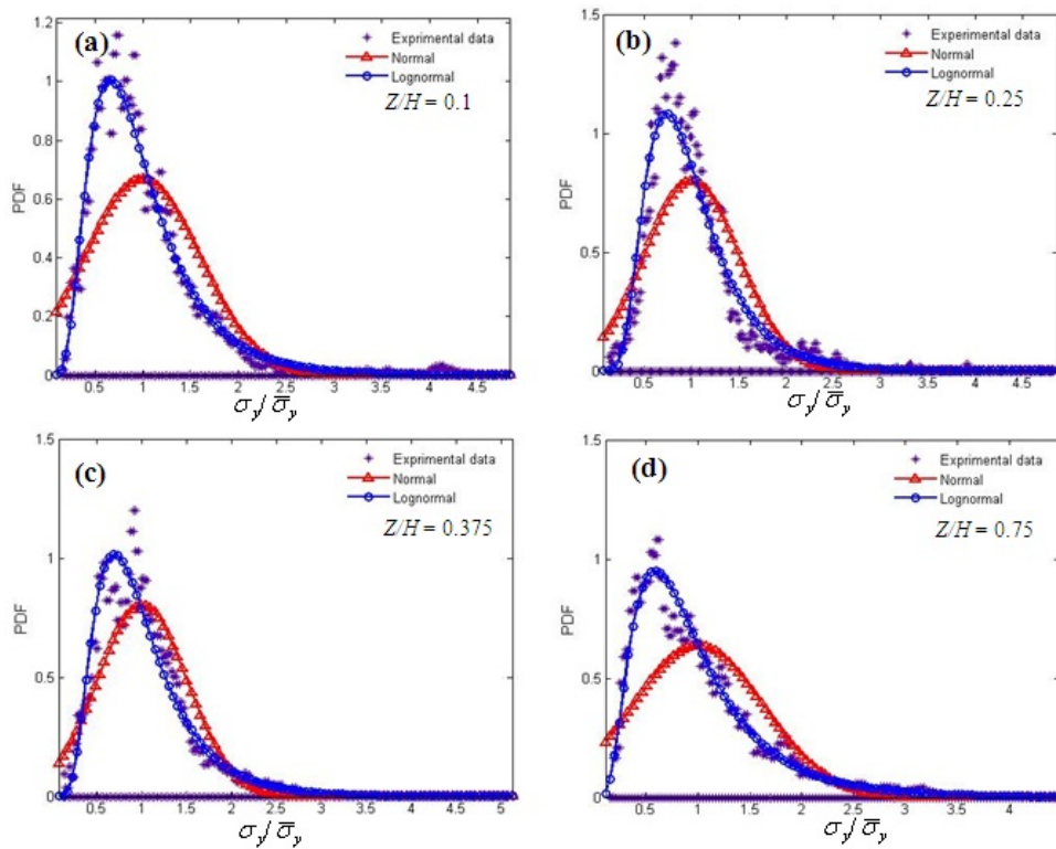
Fig. 8: Probability density for crosswind plume dispersion measured at X/H = 0.375 .
