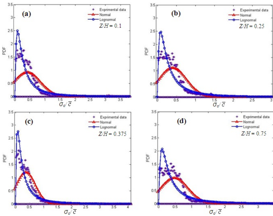
Fig. 5: Probability density for fluctuation intensity measured at X/H = 0.375 .
