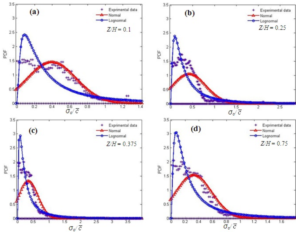
Fig. 4: Probability density for mean concentration measured at X/H = 0.625 .
