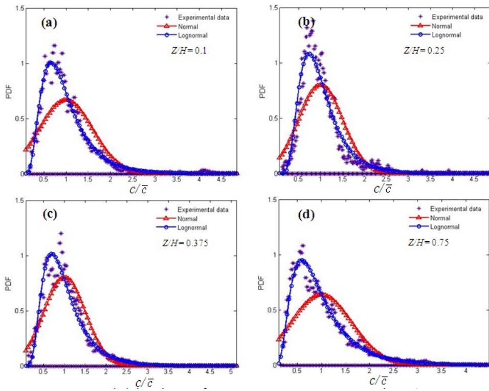
Fig. 3: Probability density for mean concentration measured at X/H = 0.625 .
