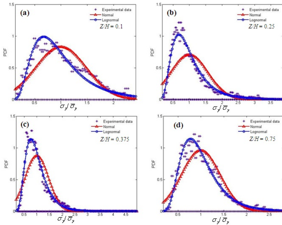
Fig. 7: Probability density for fluctuation intensity measured at X/H = 1.125 .
