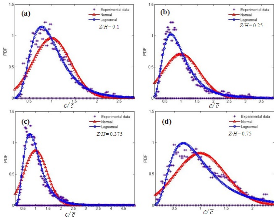
Fig. 1: Probability density for mean concentration measured at X/H = 0.375
