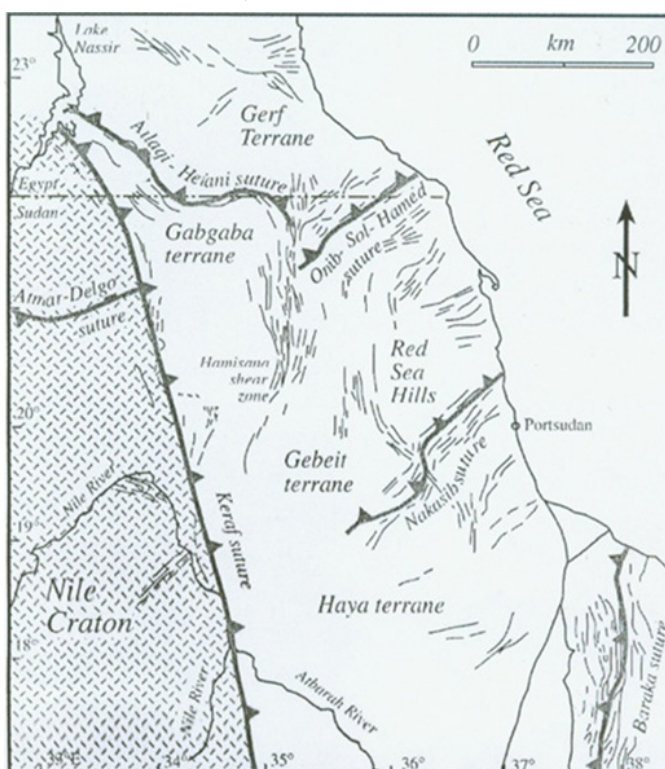
Fig. 3: Map showing the two ensimatic island arcs; Gerf and Gabgaba terranes (after Abdelsalam and Stern, 1996).
