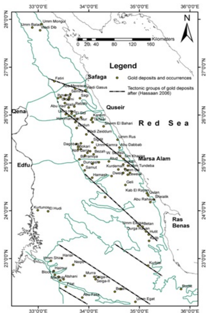
Fig. 2: Map showing the distribution of gold deposits and occurrences in the tectonic groups, Eastern Desert.
