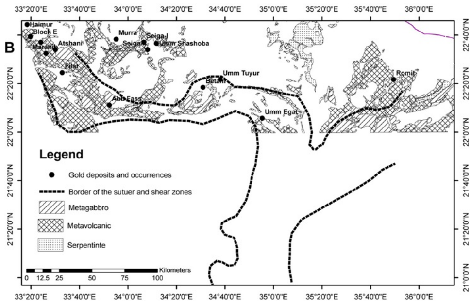
Fig. 4: Map showing the geology (after Conoco, 1987) and distribution of gold deposits and occurrences in the (Allaqi-Heiani,) – (Onib-Sol-Hamed) district.
