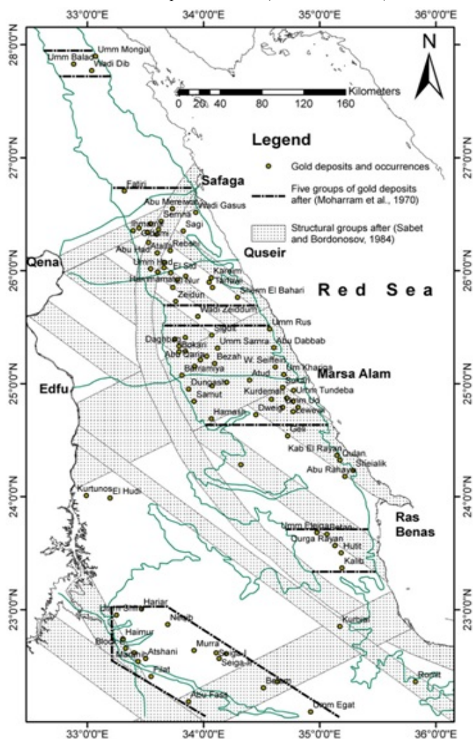
Fig. 1: Map showing the distribution of gold deposits and occurrences in the Eastern Desert.
