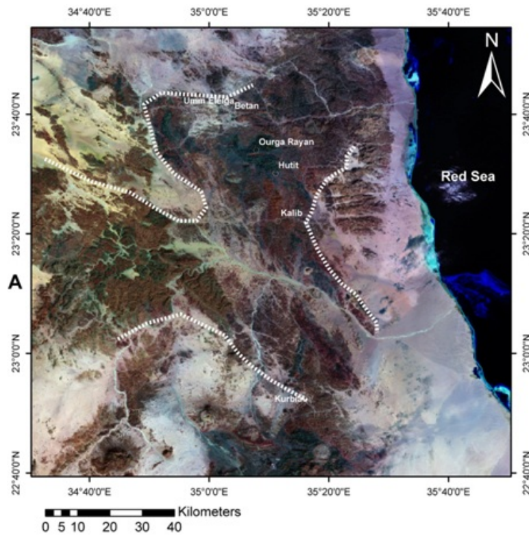
Fig. 6a: ETM+ false color image combination of bands 7, 4, 2 in (RGB) showing the distribution of gold deposits and occurrences in the Wadi Kharit- Wadi Hodein, suture (I).
