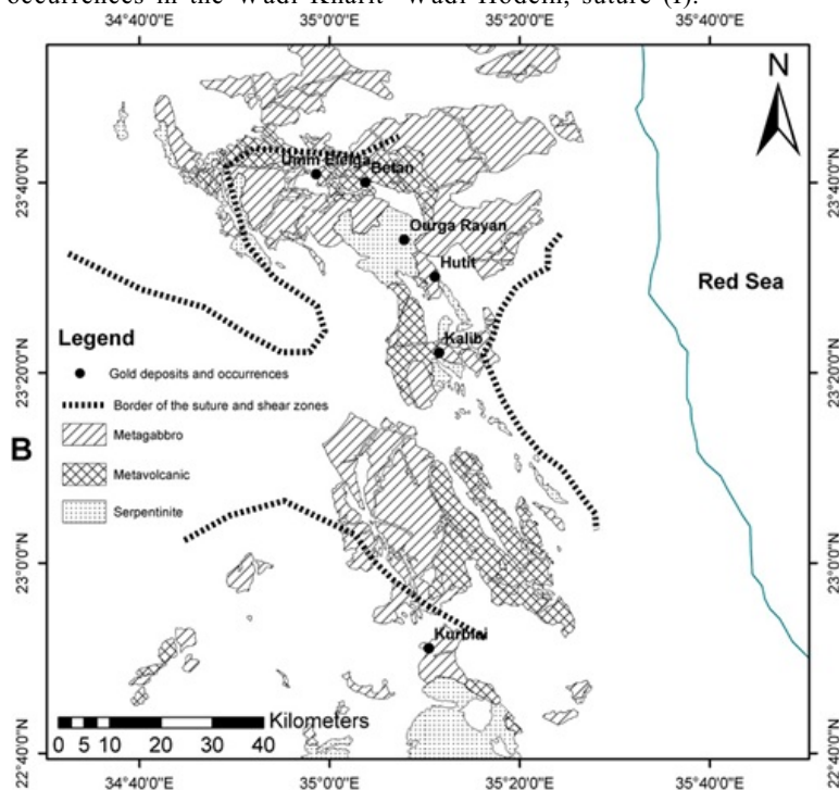
Fig. 6b: Map showing the geology (after Conoco, 1987) and distribution of gold deposits and occurrences in the Wadi Kharit- Wadi Hodein, (I) suture.
