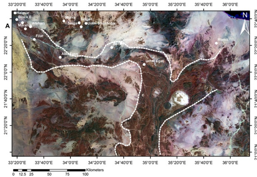
Fig. 4a: ETM+ false color image combination of bands 7, 4, 2 in (RGB) showing the distribution of gold deposits in the (Allaqi-Heiani,) – (Onib-Sol-Hamed) suture zones.
