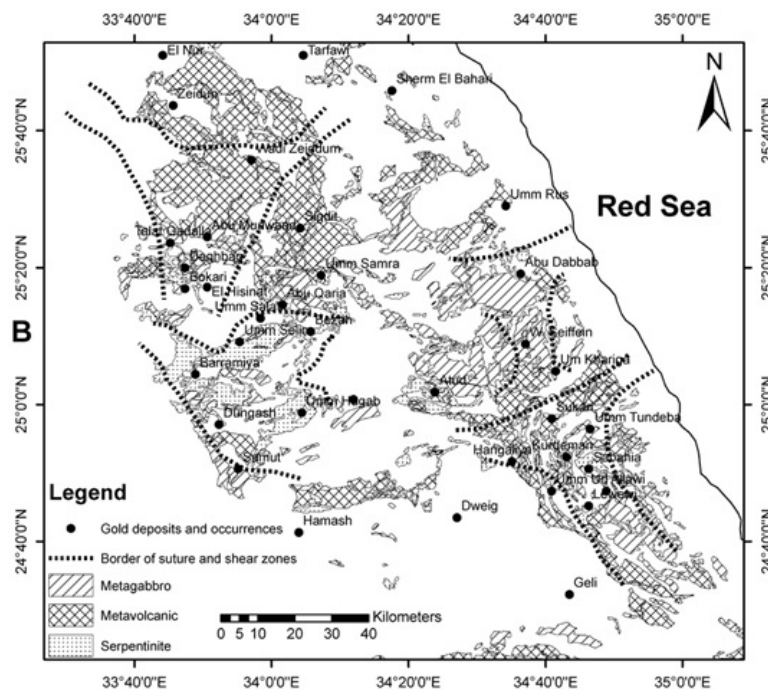
Fig. 7b: Map showing the geology (after Conoco, 1987) and distribution of gold deposits and occurrences in the II, III, IV, and V suture and shear zones.
