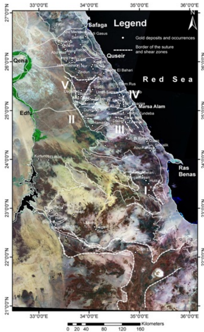
Fig. 5: Google Earth false color image showing the distribution of gold deposits and occurrences and borders of Allaqi-Heiani and Onib-Sol Hamed and the 5 recorded suture and shear zones in the Nubian Shield, Eastern Desert.
