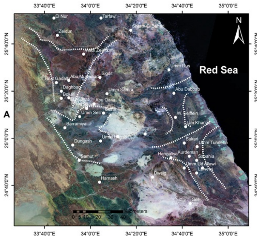
Fig. 7a: ETM+ false color image combination of bands 7, 4, 2 in (RGB) showing the distribution of gold deposits and occurrences in the Barramiya (II), Atud-Sukari (III), Um Khariga-Wadi Abu Dabbab (IV) and Talaat Gadallah-Um Samara (V) suture and shear zones (for location No. see Fig. 5).
