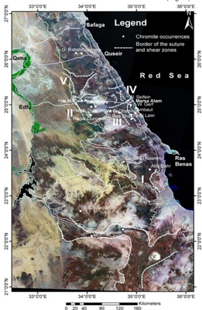
Fig. 8: ETM+ false color image combination of bands 7, 4, 2 in (RGB) showing the distribution of chromite occurrences and borders of the 5 recorded suture and shear zones in the Nubian Shield, Eastern Desert.
